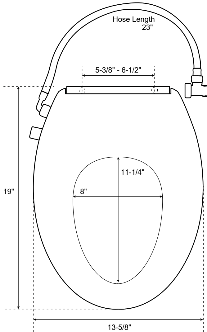
Elongated Seat Dimensions
